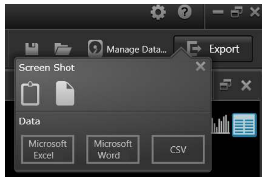
Figure 5. Export menu
